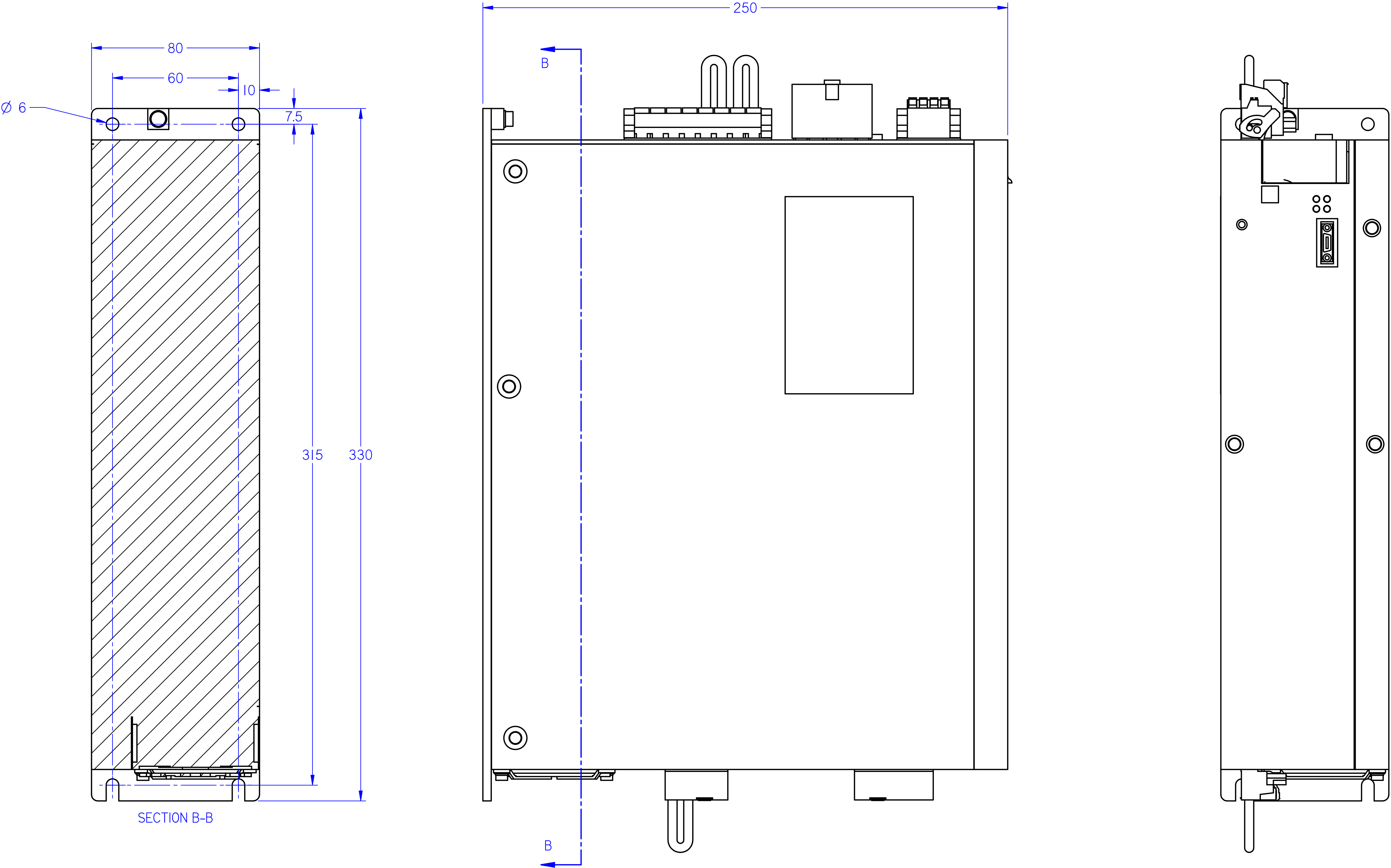
Drive Mounting Holes
